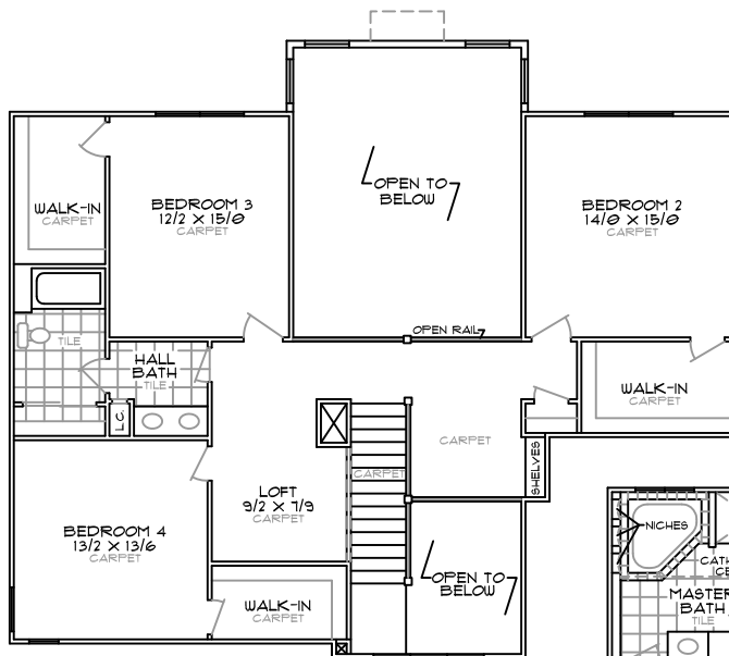
SECOND FLOOR PLAN - 1282 sq. ft.
