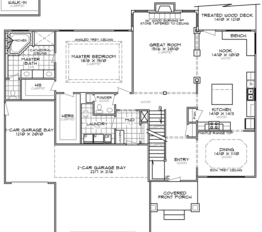
MAIN FLOOR PLAN - 1910 sq. ft.
